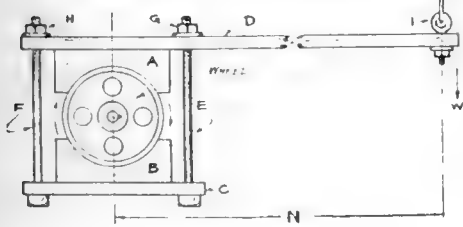
The brake horsepower of a motor can be accurately measured by means of a simple apparatus such as the one here shown
